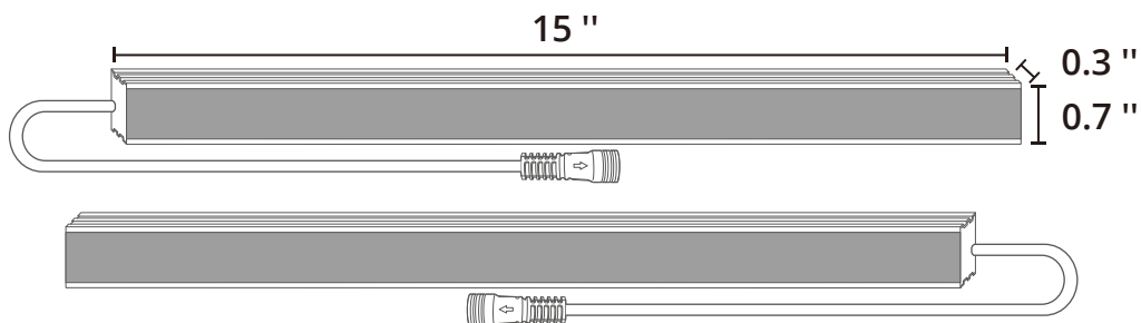
Trailer Light Bar
