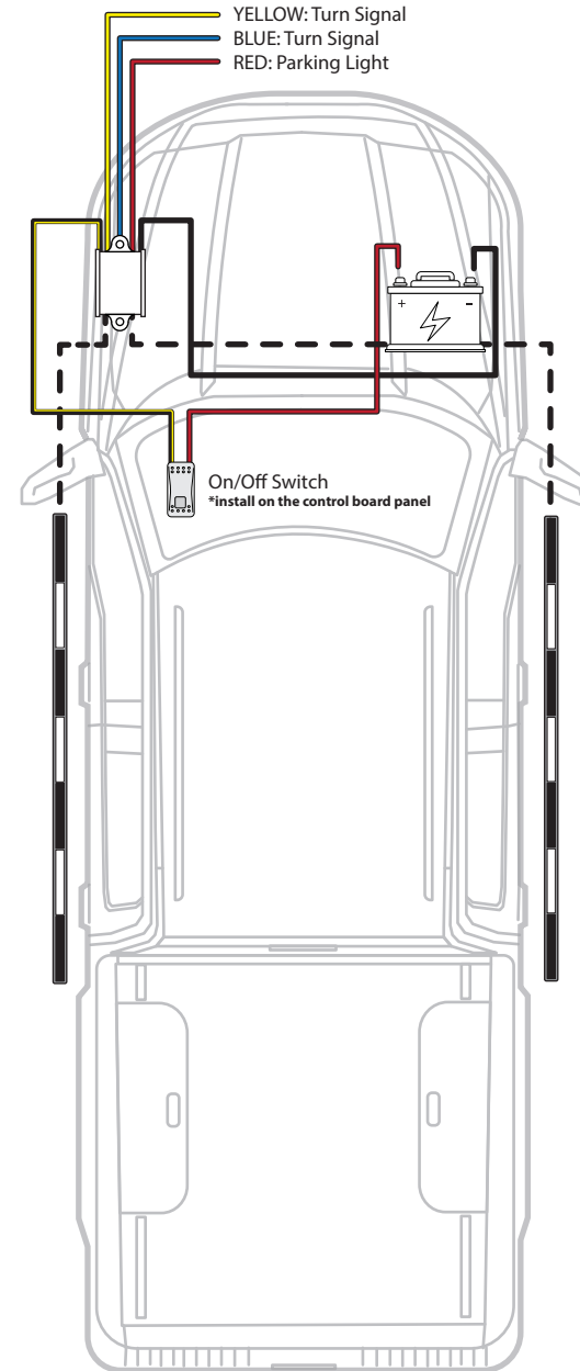
WIRE AND INSTALL LOCATION SUGGESTION
